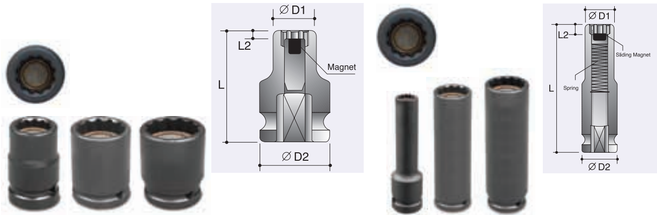
12-Point Sockets
