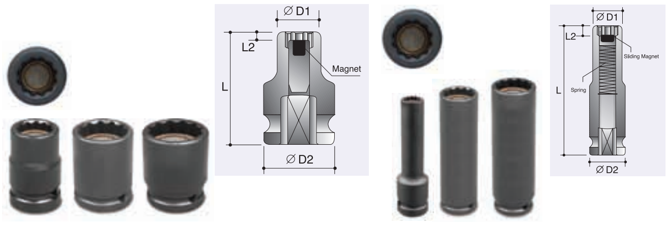
12-Point Sockets
