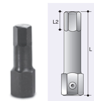
Hex Drivers
